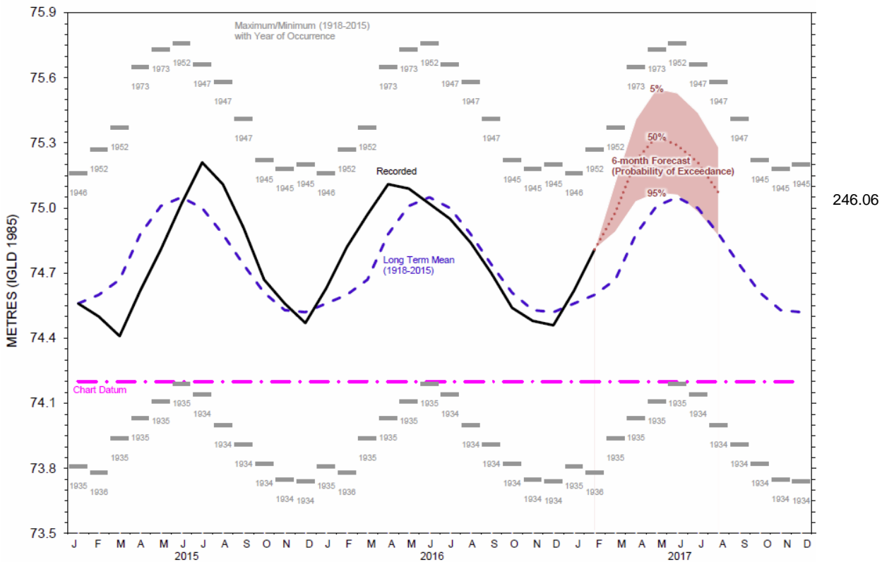
LAKE ONTARIO MONTHLY MEAN LEVELS
